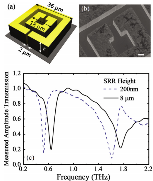
FIG. 1. (Color online) (a) Schematic diagram of a SRR illustrating the dimensions used in this study and the SRR height parameter ( h ), (b) electron micrograph of high aspect ratio SRR with h=8\ \mu\text{m} (scale bar= 2\ \mu\text{m} ), and (c) measured THz spectra for SRRs of different heights.
